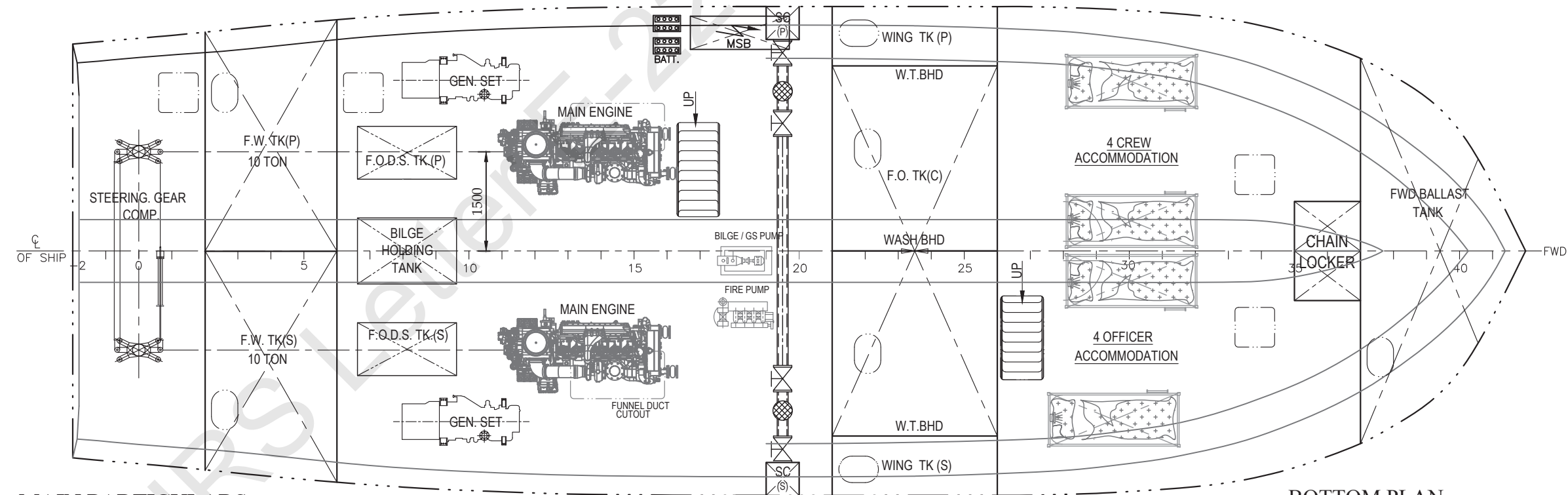
BOTTOM PLAN
